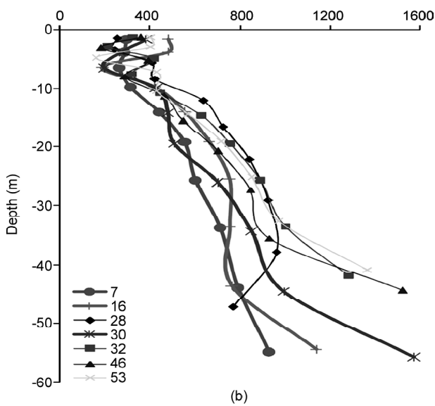
Figure 13. Shear wave velocity profiles corresponding to class C site as per NEHRP Vs 30 .
